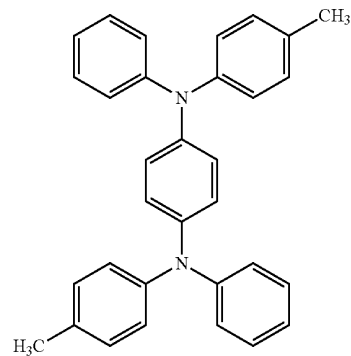
N,N'-Diphenyl-N,N'-di-p-tolylbenzene-1,4-diamine
