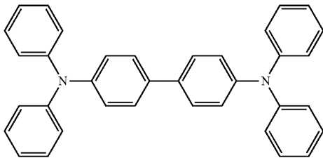
Tetra-N-phenylbenzidine
