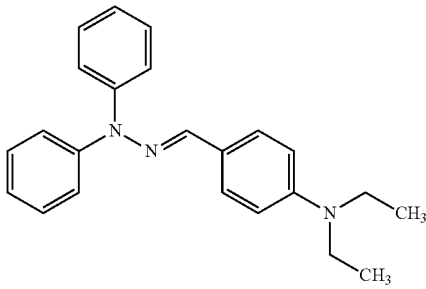
4-(Diethylamino)benzaldehyde diphenylhydrazone
