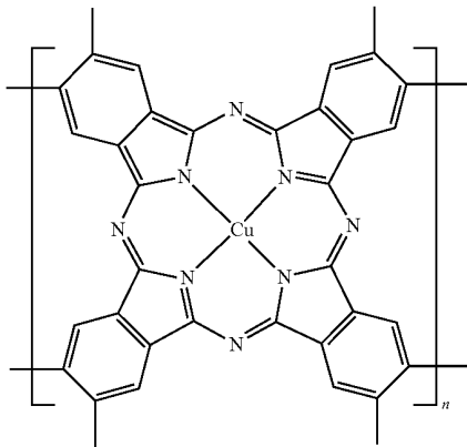
Poly(copper phthalocyanine)
