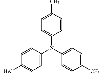
Tri-p-tolylamine
