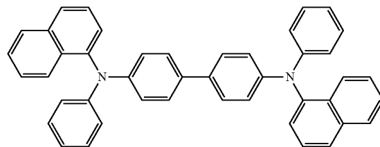
N,N'-Di-[(1-naphthyl)-N,N'-diphenyl]-1,1'-biphenyl-4,4'-diamine
