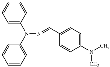
4-(Dimethylamino)benzaldehyde diphenylhydrazone
