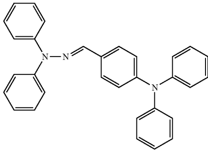
4-(Diphenylamino)benzaldehyde diphenylhydrazone
