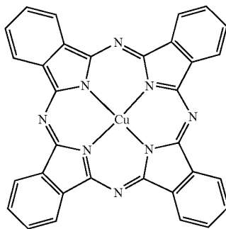
Copper(II) phthalocyanine
