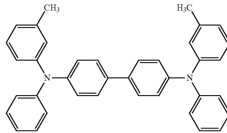
N,N'-Bis(3-methylphenyl)-N,N'-diphenylbenzidine
