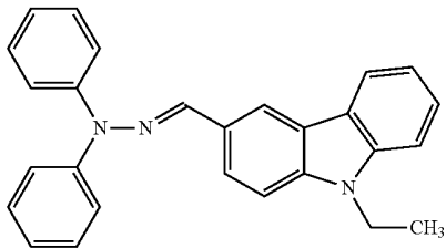
9-Ethyl-3-carbazolecarboxaldehyde diphenylhydrazone
