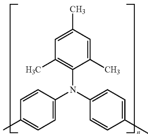
Poly[bis(4-phenyl)(2,4,6-trimethylphenyl)amine]
