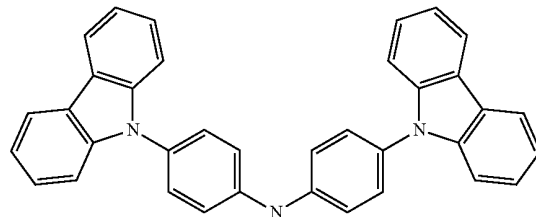
Tri-p-tolylamine
